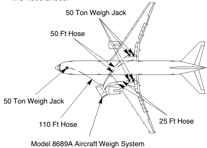
Typical Wide Body Aircraft Weigh System Application
