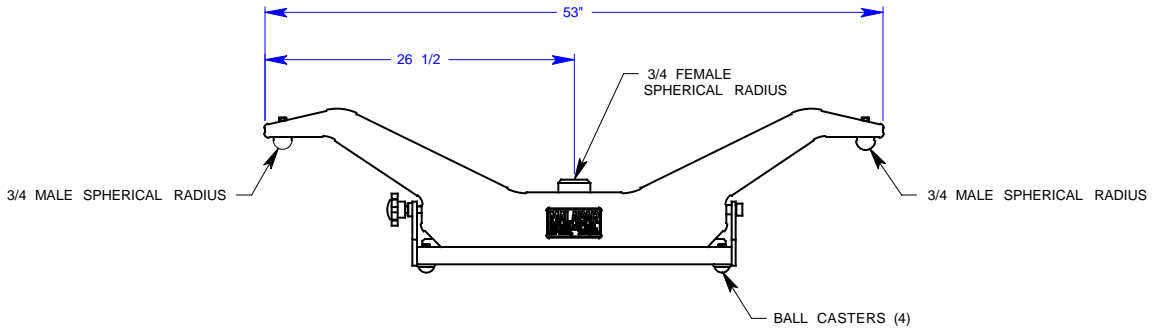
BEAM SHOWN IN JACKING POSITION
